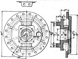
Figs. 928-930. Back Cylinder Head. American Locomotive Co.
